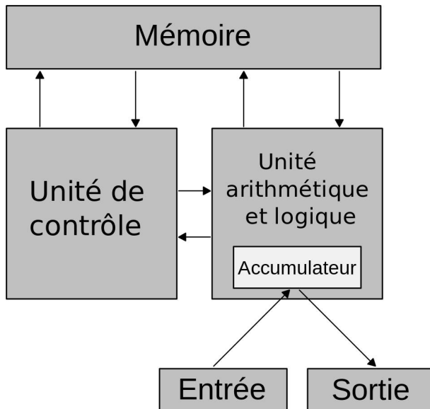
FIGURE 8 – Architecture de von Neumann
