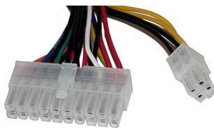
FIGURE 51 – ATX 20+4
