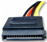
FIGURE 54 – Alimentation SATA
